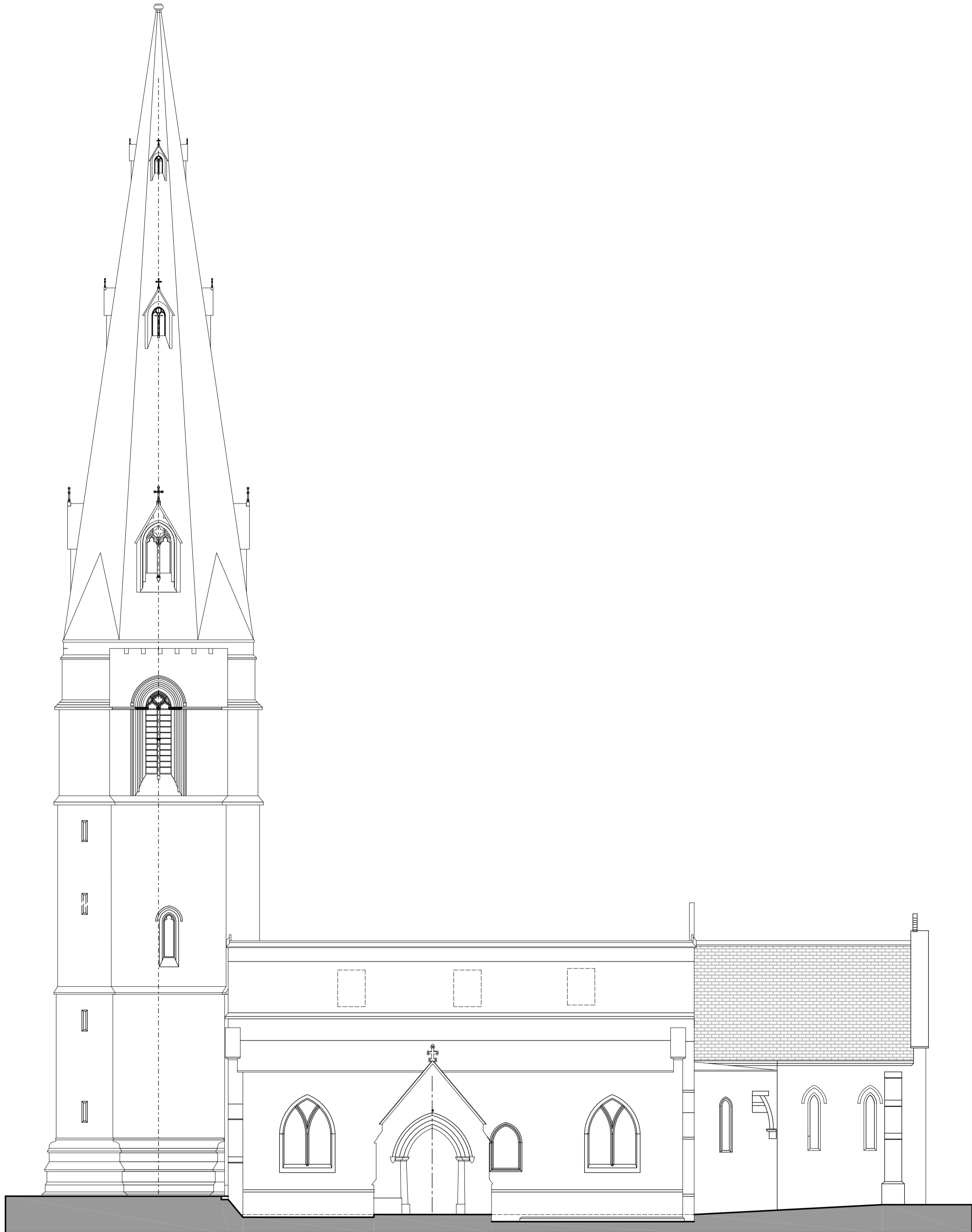
South Elevation 1:100
